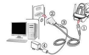
RS232 cable
